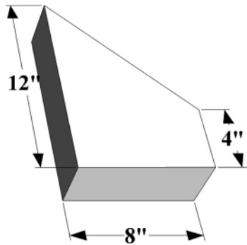
45° Corner Miter Cuts (4 Pieces)
