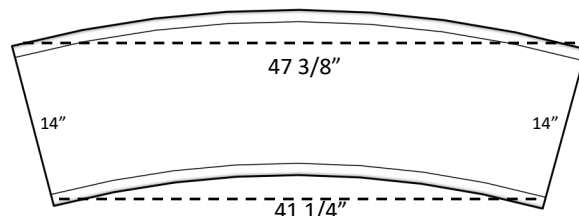
Natural Stone Cap(6)
